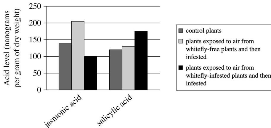
Jasmonic and Salicylic Acid Levels in Tomato Plants
